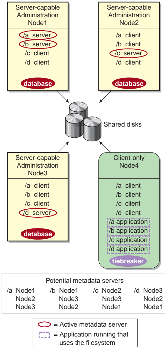
Figure 1-5 Three Metadata Servers for Four Filesystems
