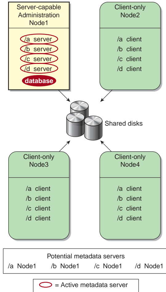
Figure 1-3 One Metadata Server (No Relocation or Recovery)
