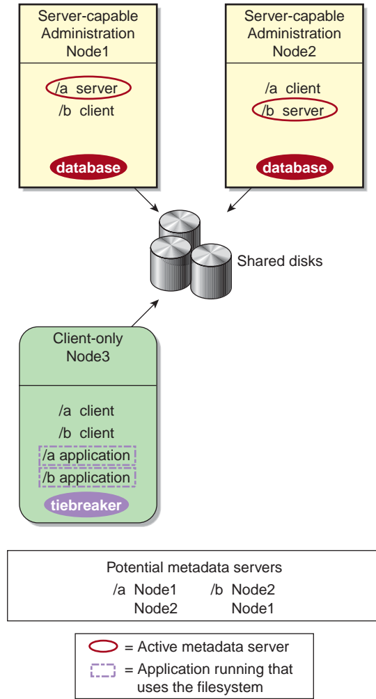
Figure 1-4 Two Metadata Servers for Two Filesystems
