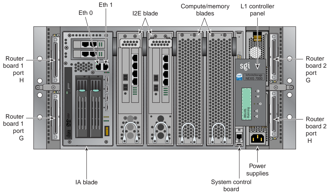
Figure 1-2 SGI InfiniteStorage NEXIS 7000 Compute Appliance Connectors Example
