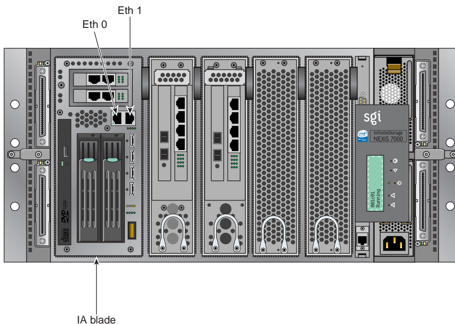
Figure 1-3 Ethernet Connection Example to Compute Appliance
