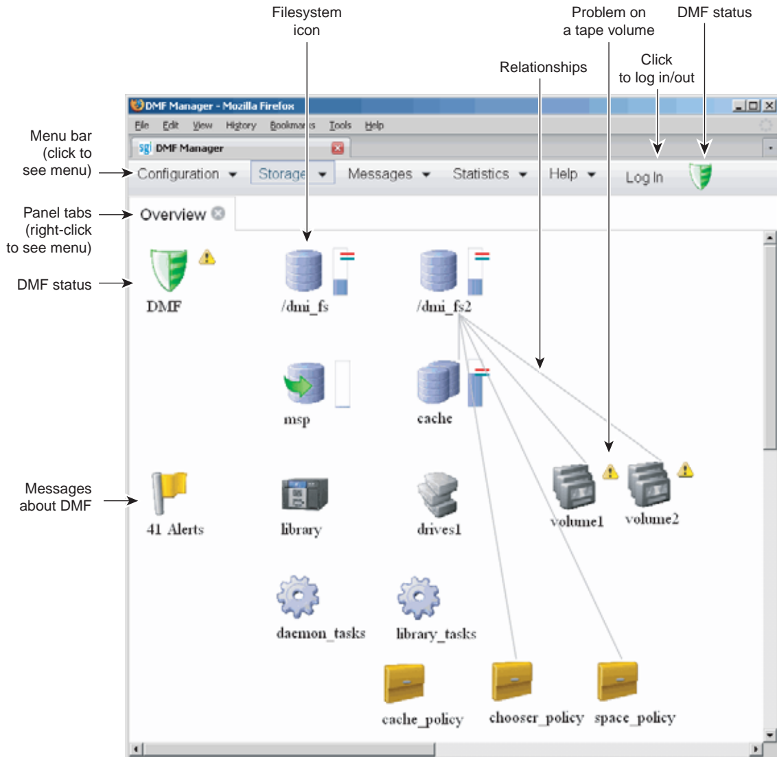
Figure 1-6 DMF Manager
